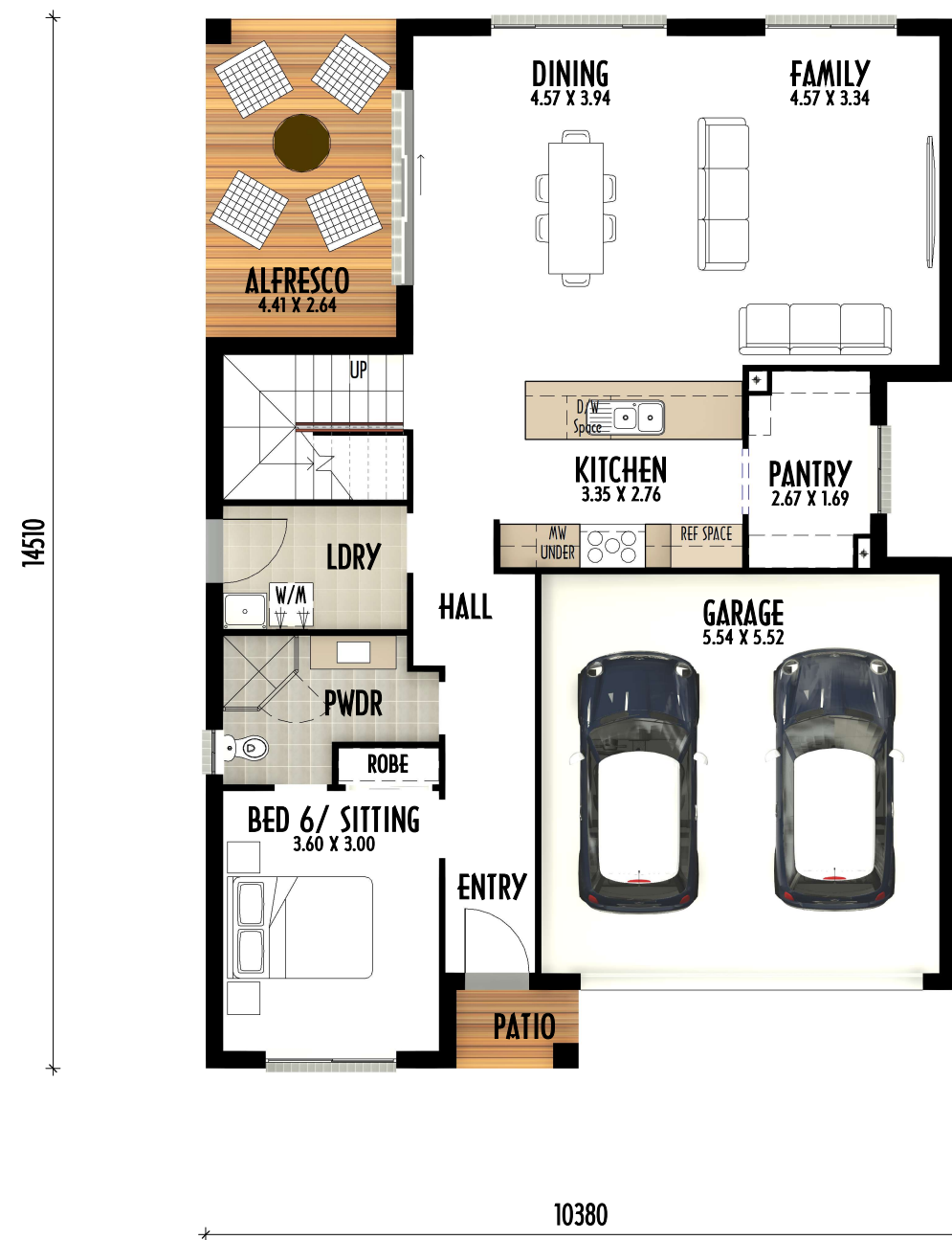
GROUND FLOOR
