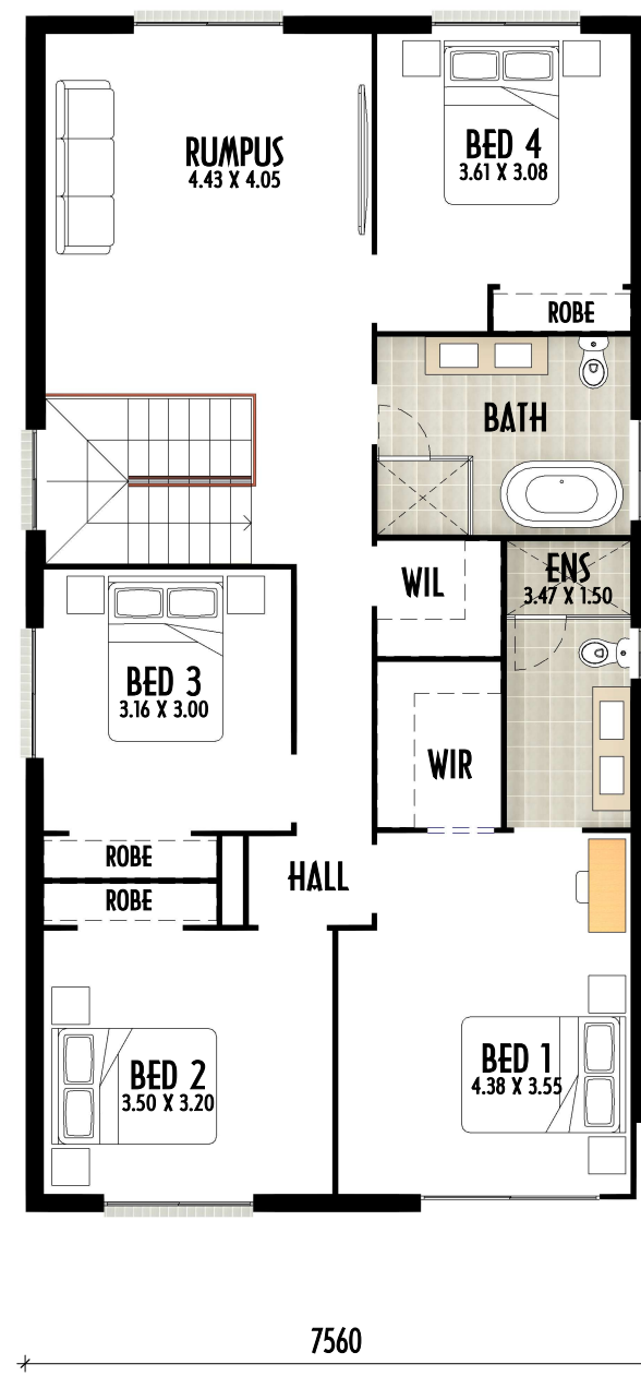
FIRST FLOOR
