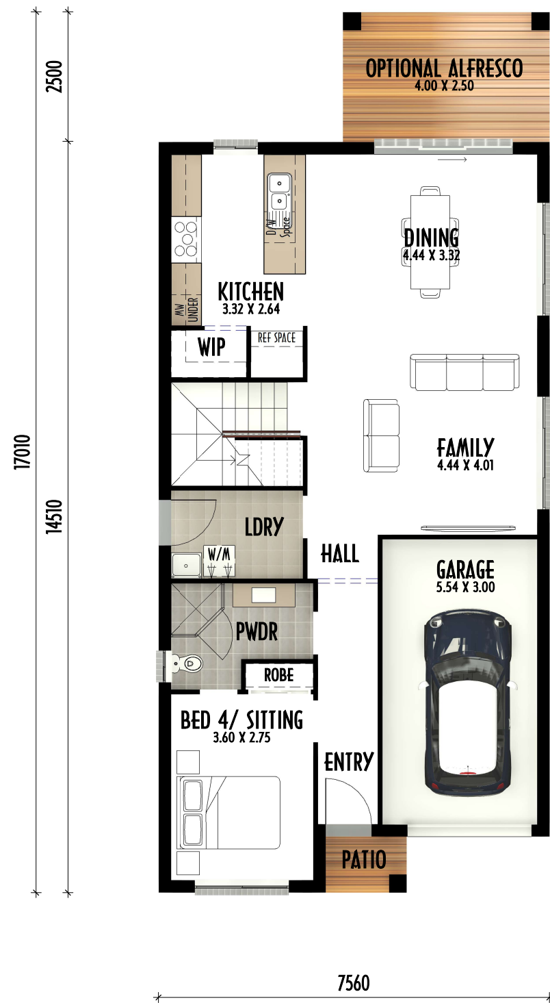
GROUND FLOOR
