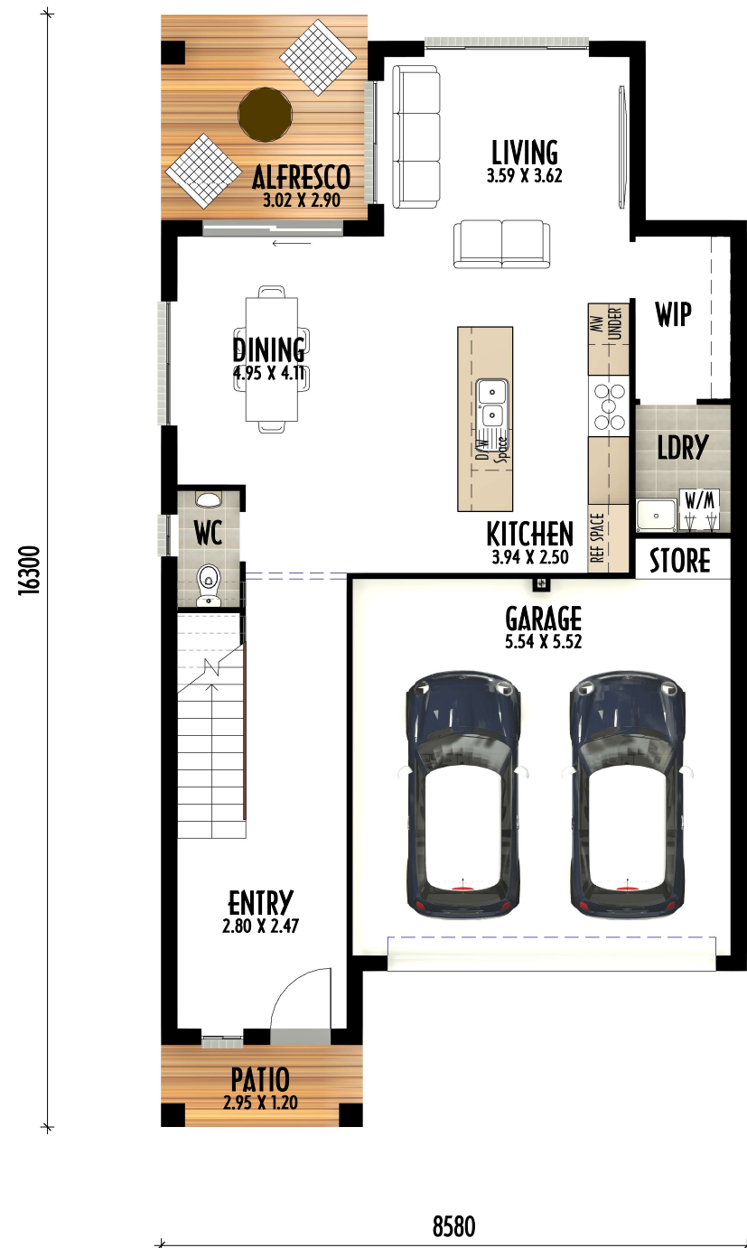
GROUND FLOOR
