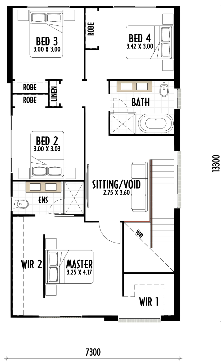
FIRST FLOOR
