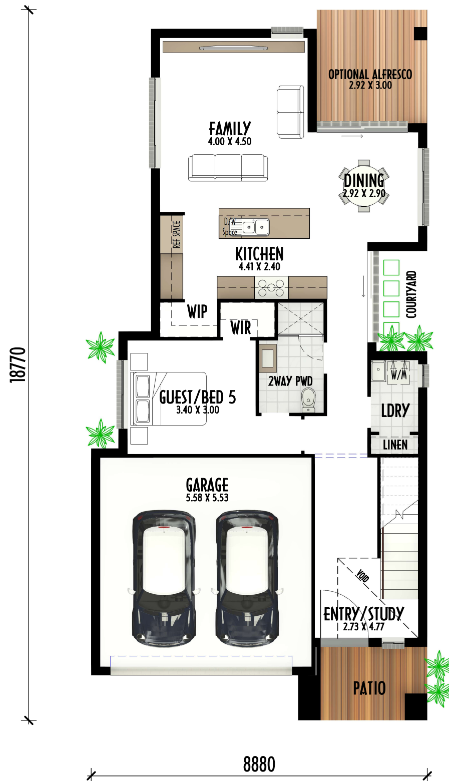
GROUND FLOOR
