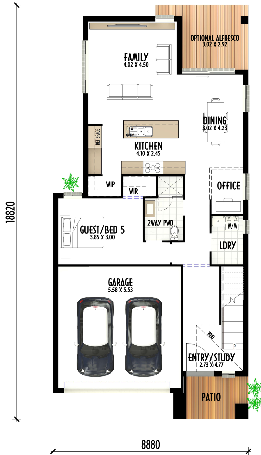
GROUND FLOOR
