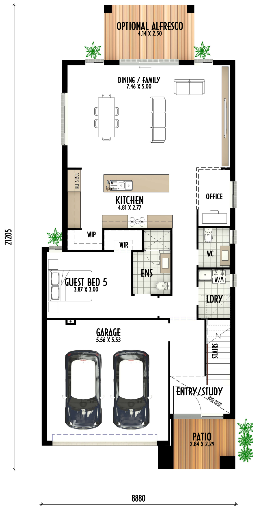
GROUND FLOOR
