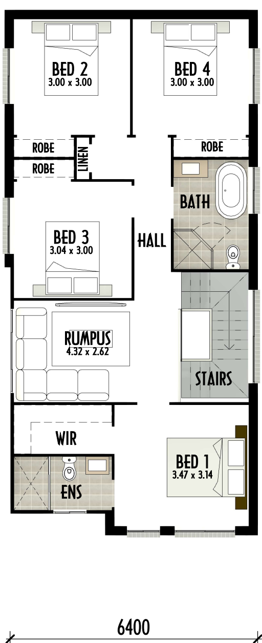
FIRST FLOOR
