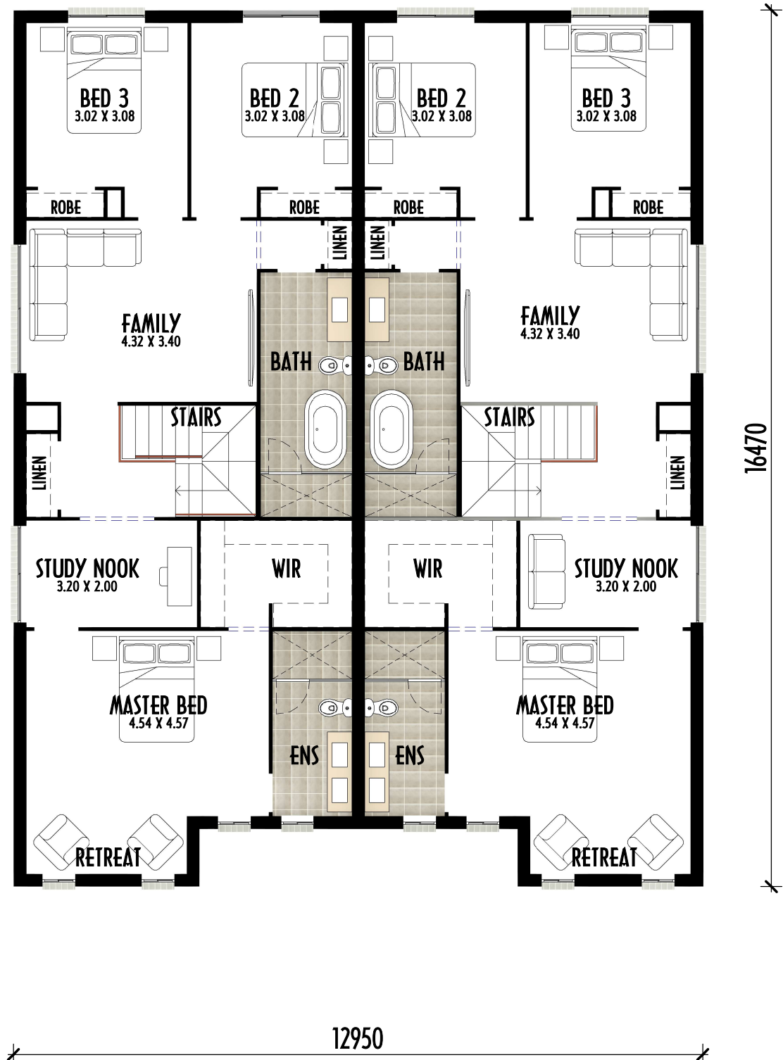
First Floor
