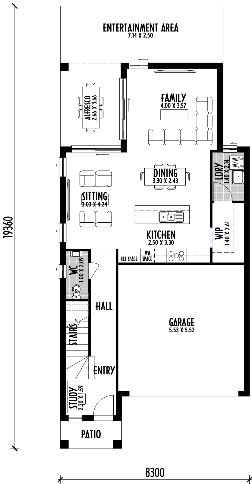
GROUND FLOOR
